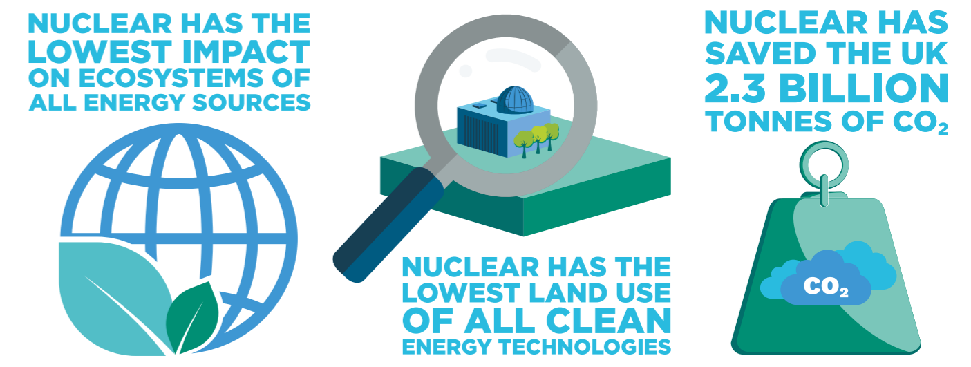
UNECE Life Cycle Assessment of Electricity Generation Options; NIA analysis of historical grid data
