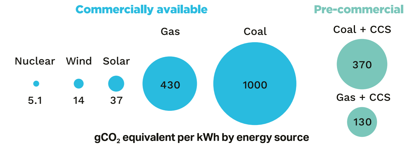
UNECE, Lifecycle CO 2 emissions of electricity generation technologies
